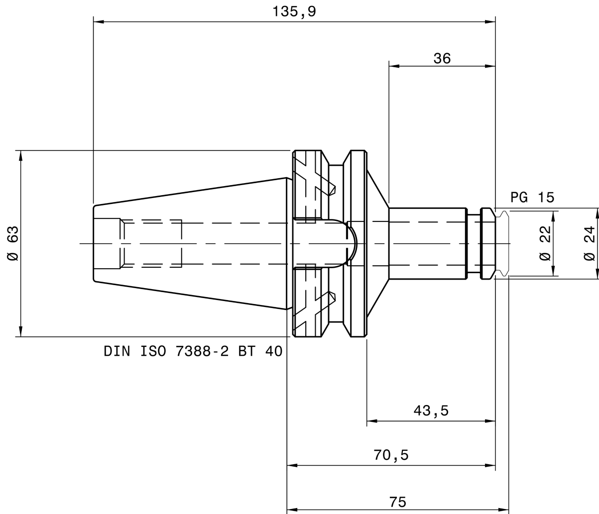
REGO-FIX B 2140.71533
