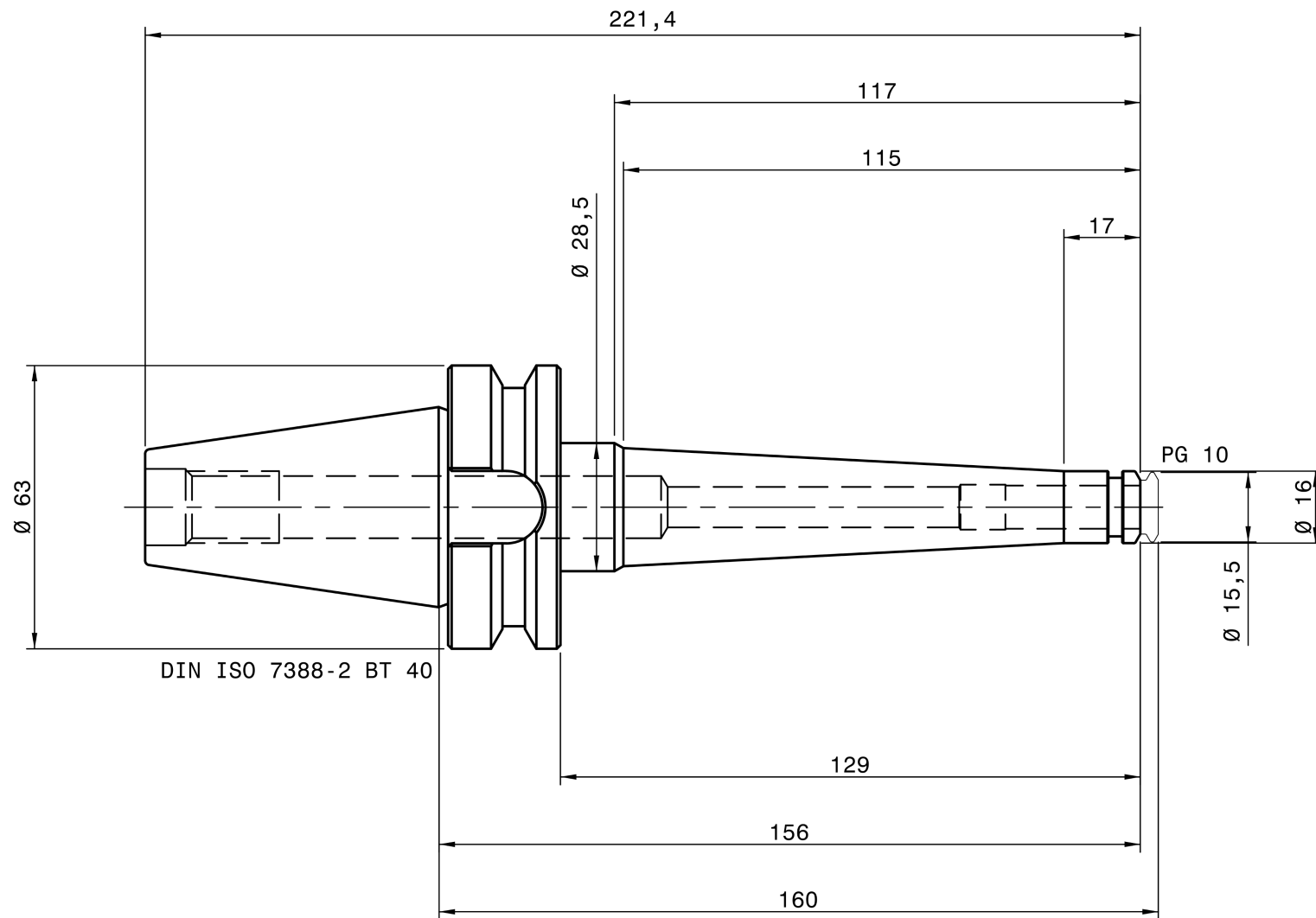
REGO-FIX 4140.71080
