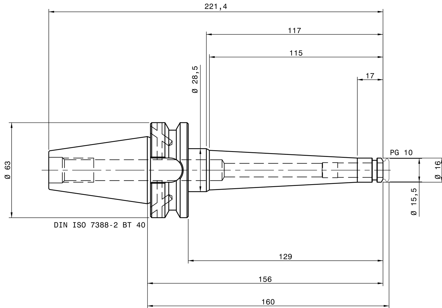
REGO-FIX B 4140.71083
