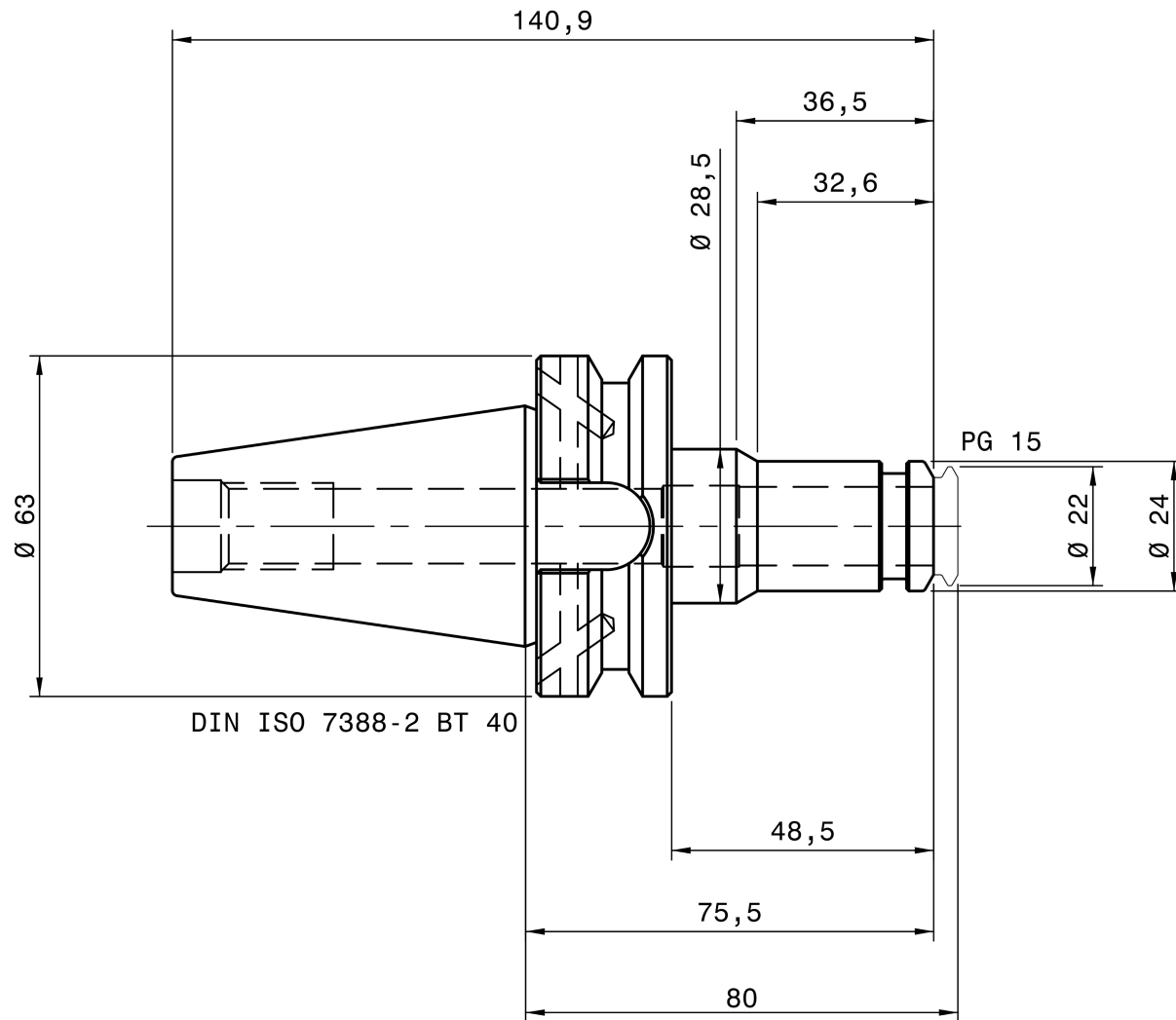
REGO-FIX B 4140.71543
