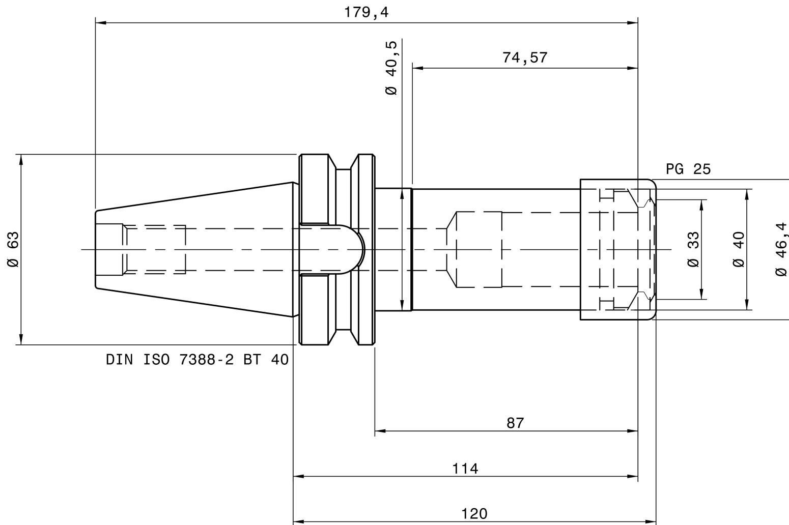
REGO-FIX SG 5140.72560
