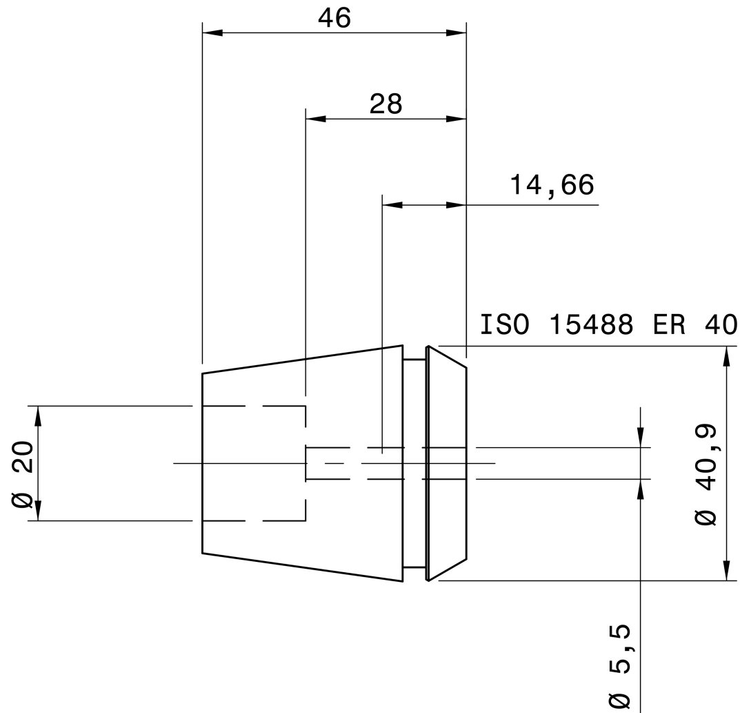
REGO-FIX 1140.05500
