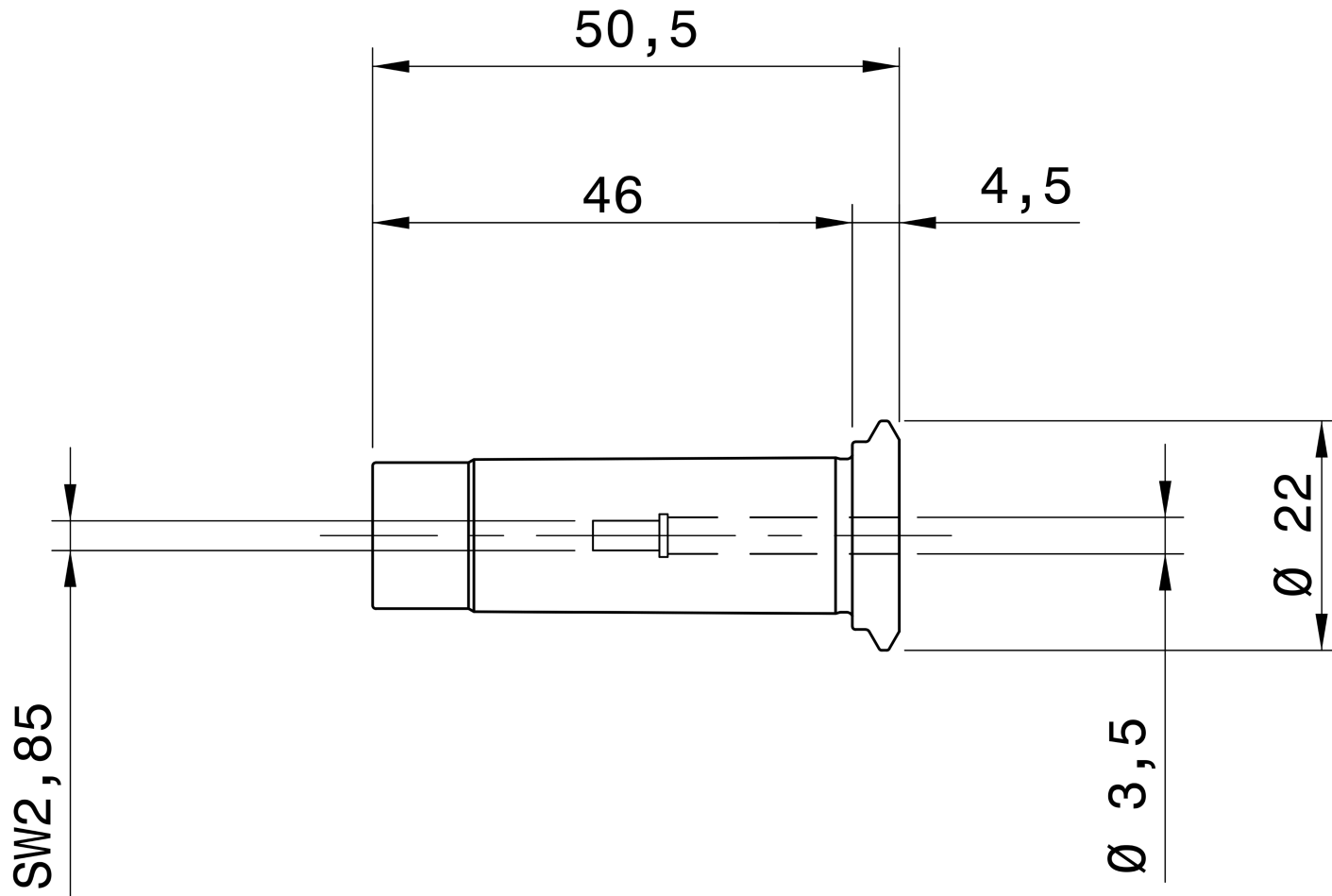
REGO-FIX 1715.03505
