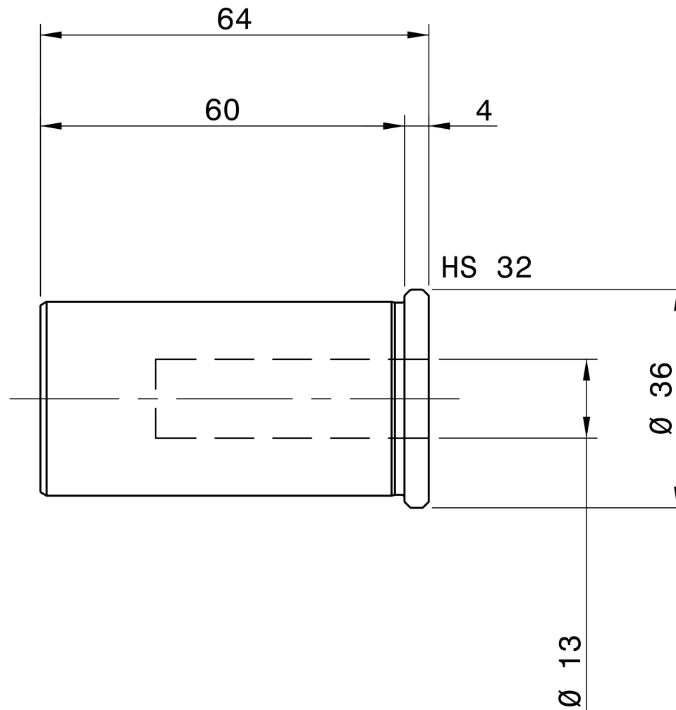
REGO-FIX 1932.13000
