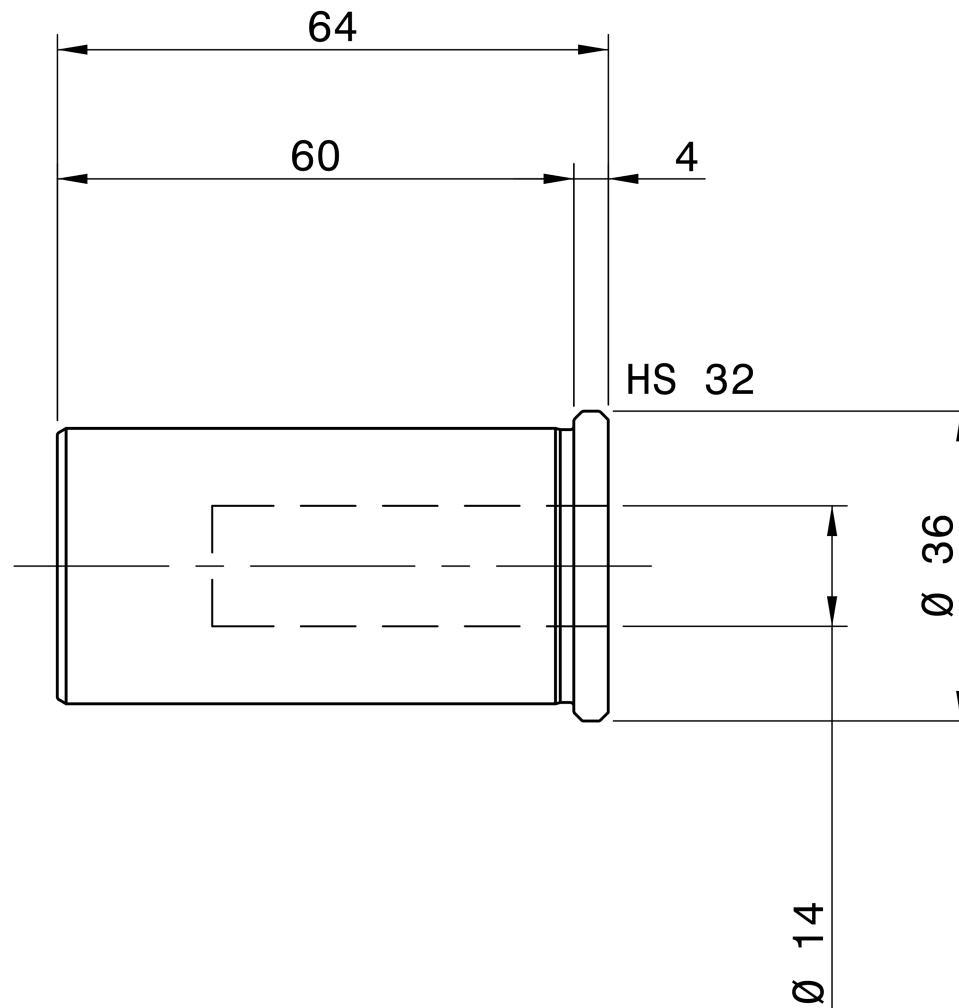
REGO-FIX 1932.14002
