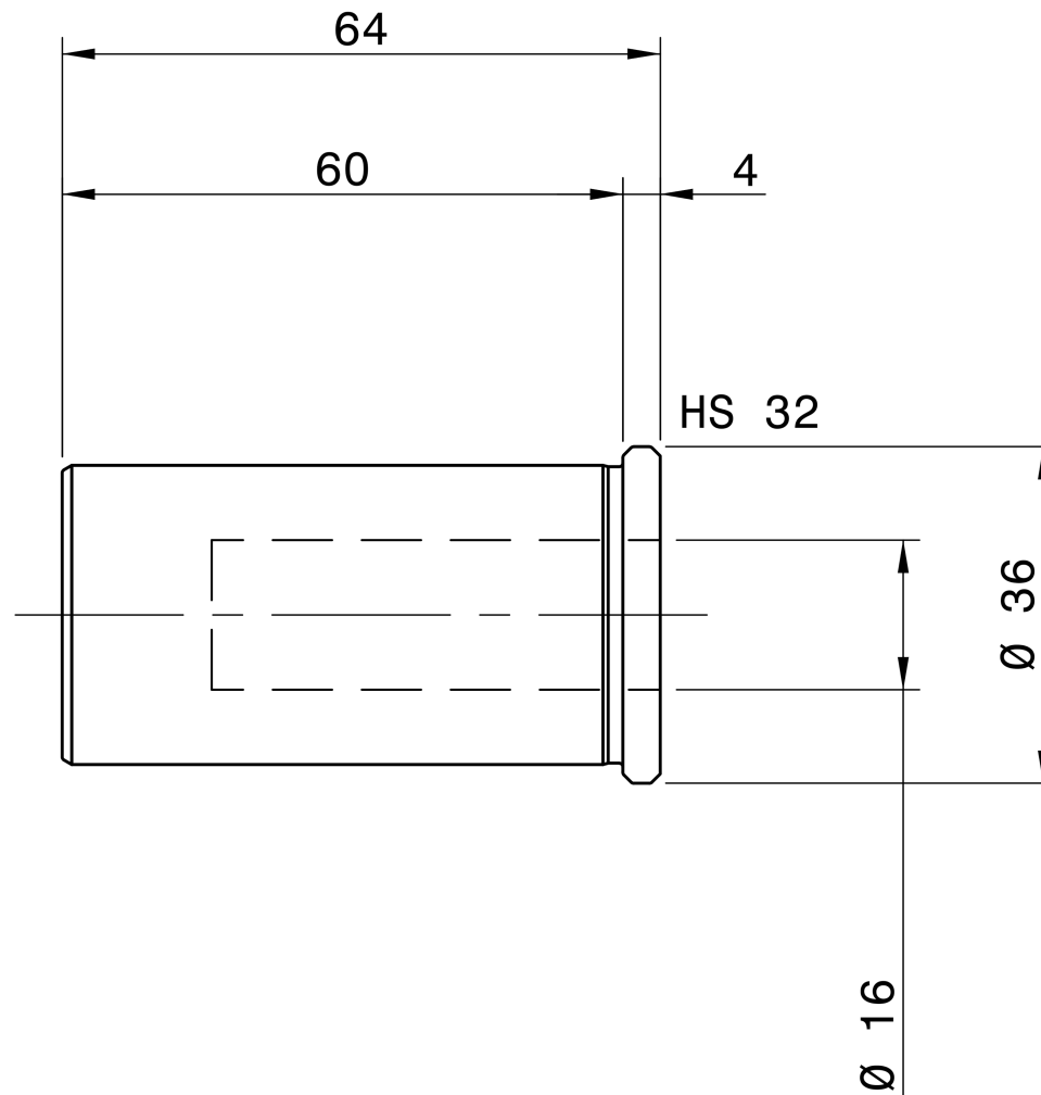
REGO-FIX 1932.16000
