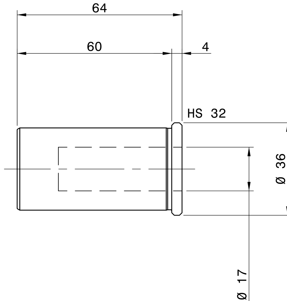
REGO-FIX 1932.17000
