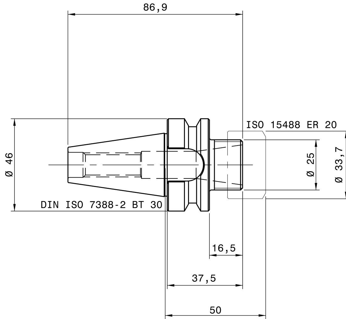
REGO-FIX 2130.12016
