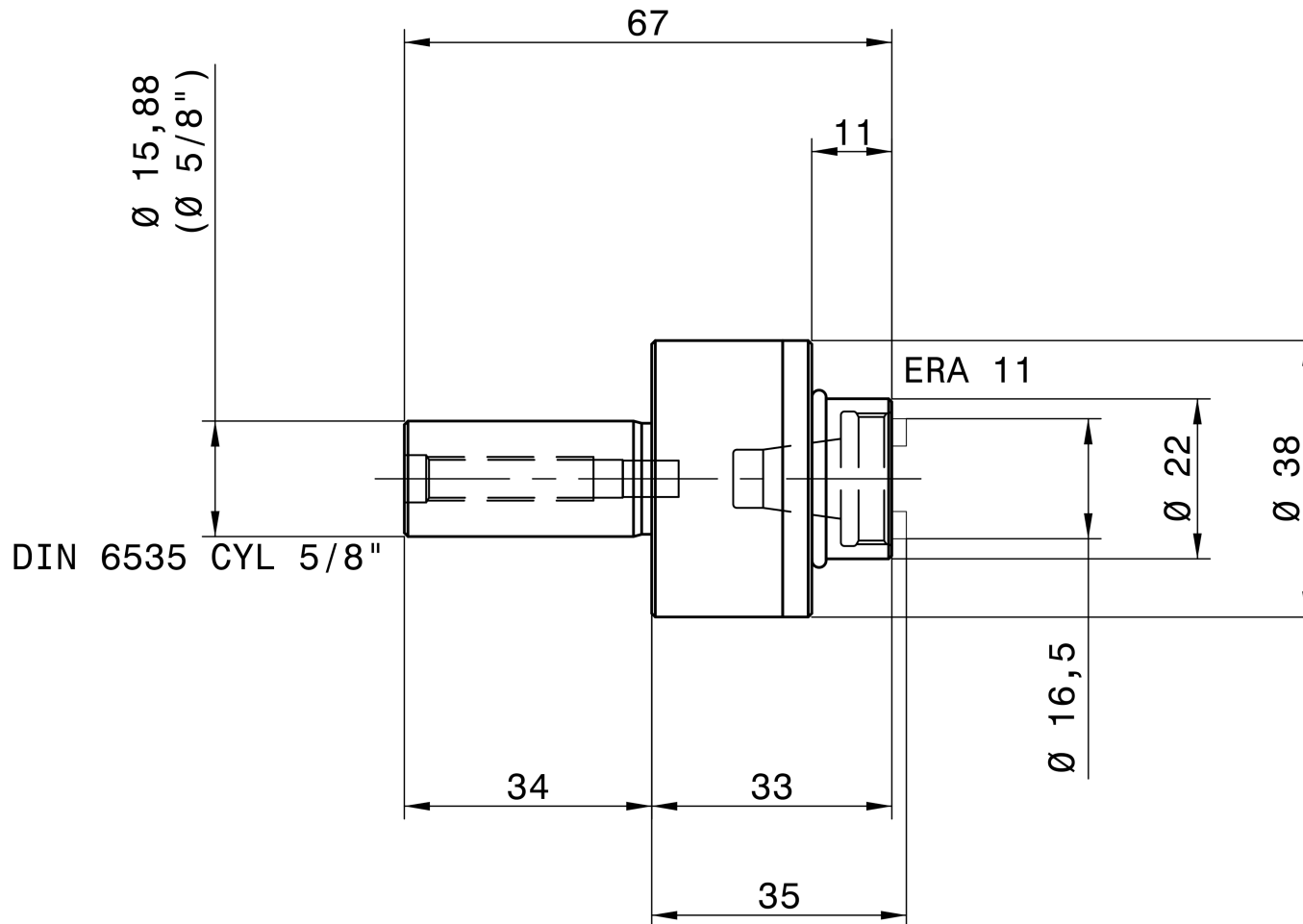
REGO-FIX 2616.91102
