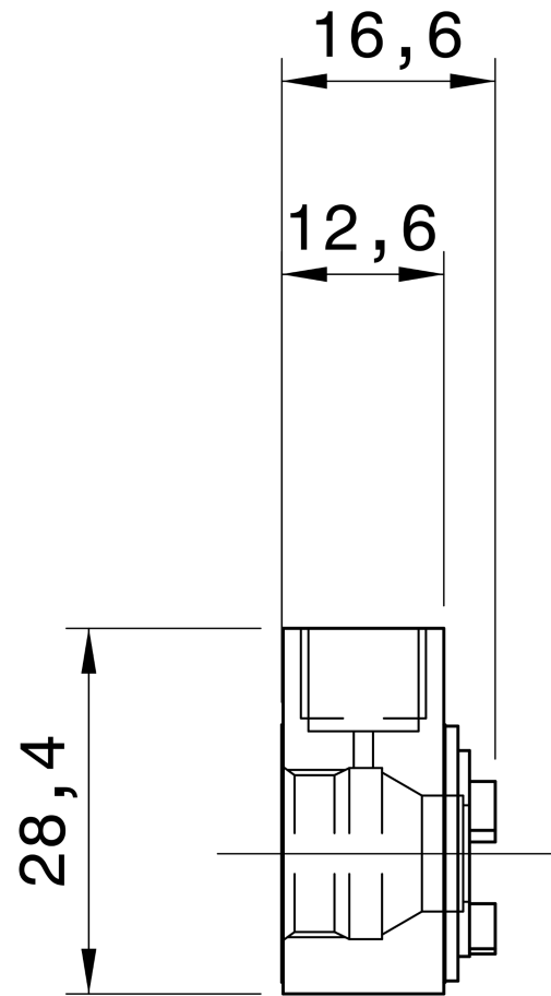
ISO 15488 ERM 11 REGO-FIX Hi-S 3711.79000
