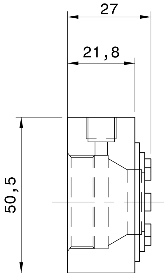
ISO 15488 ERM 25 REGO-FIX 3725.39000
