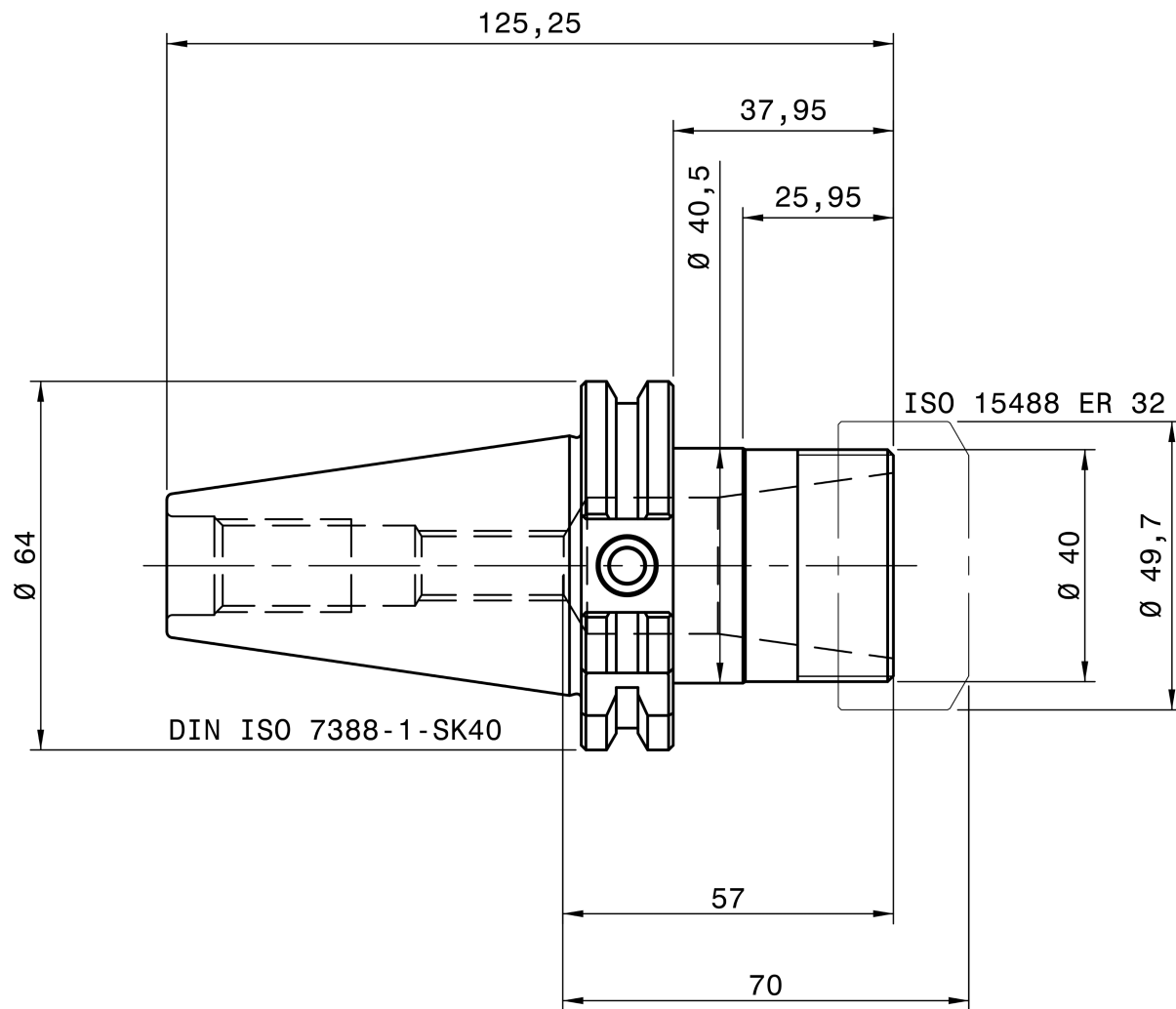
REGO-FIX B 4240.13233
