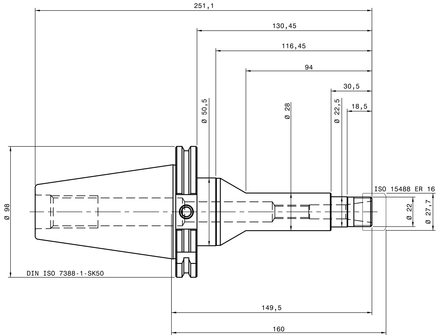
REGO-FIX B 4250.11683
