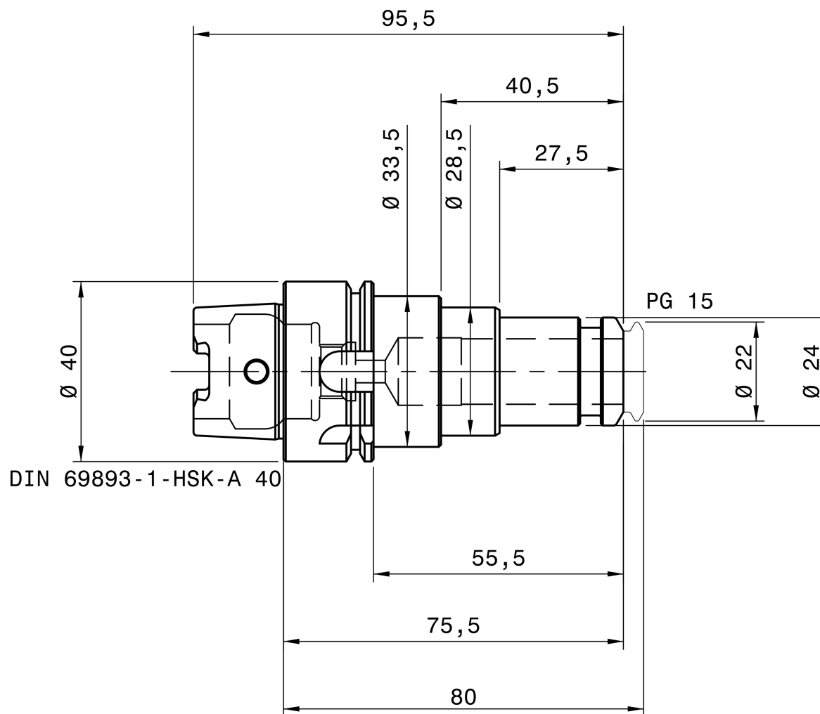
REGO-FIX 4540.71540
