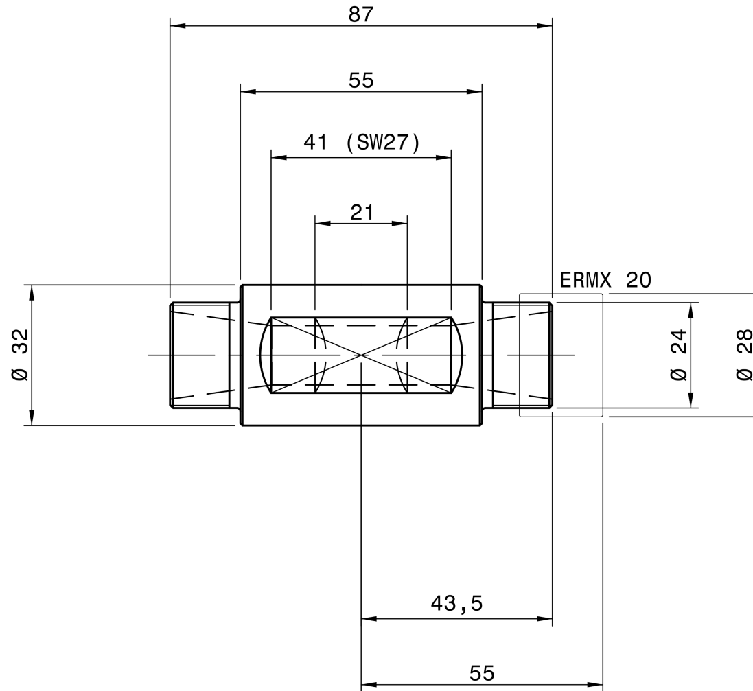
REGO-FIX 4632.22034
