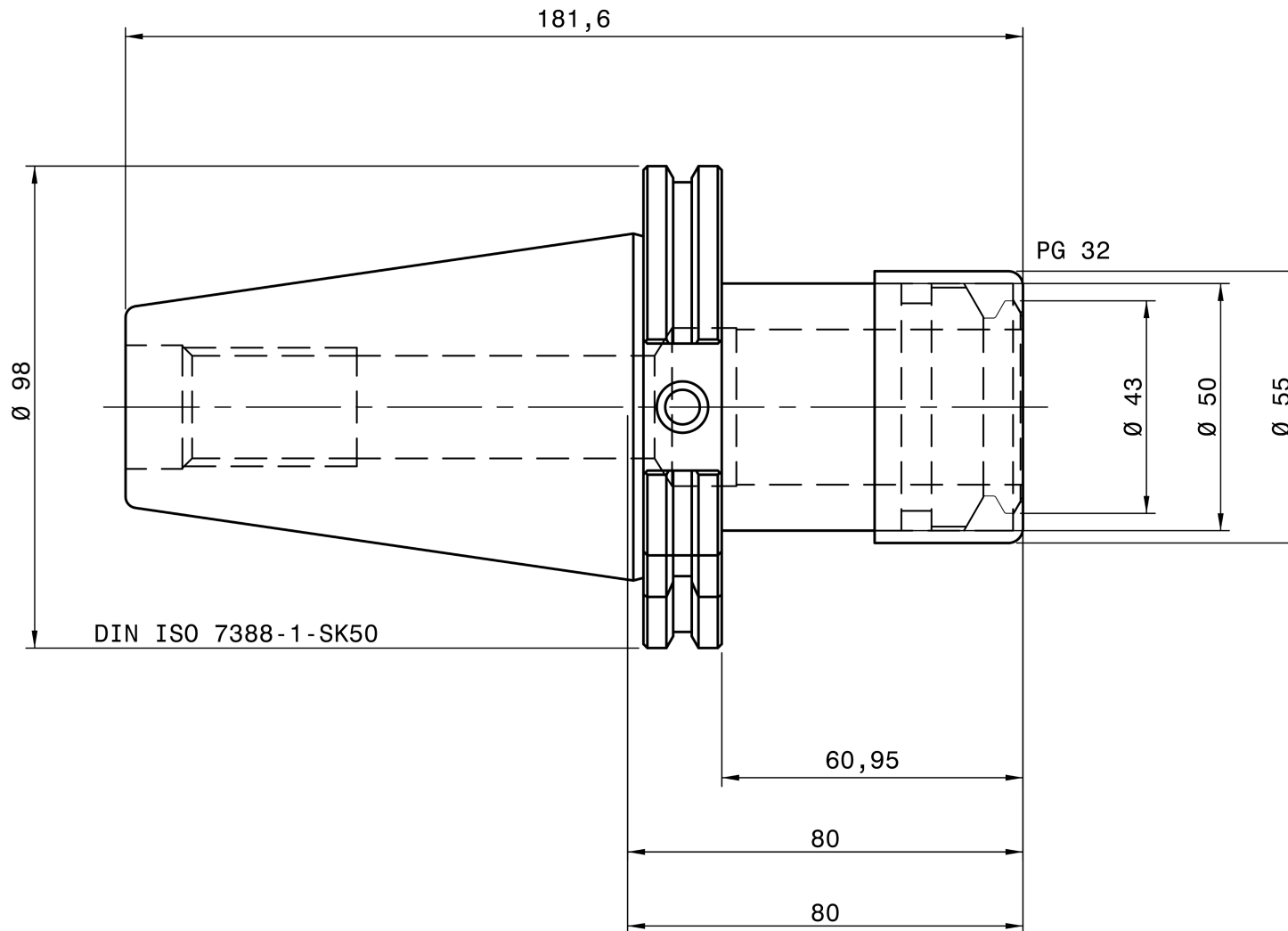
REGO-FIX SG 5250.73240
