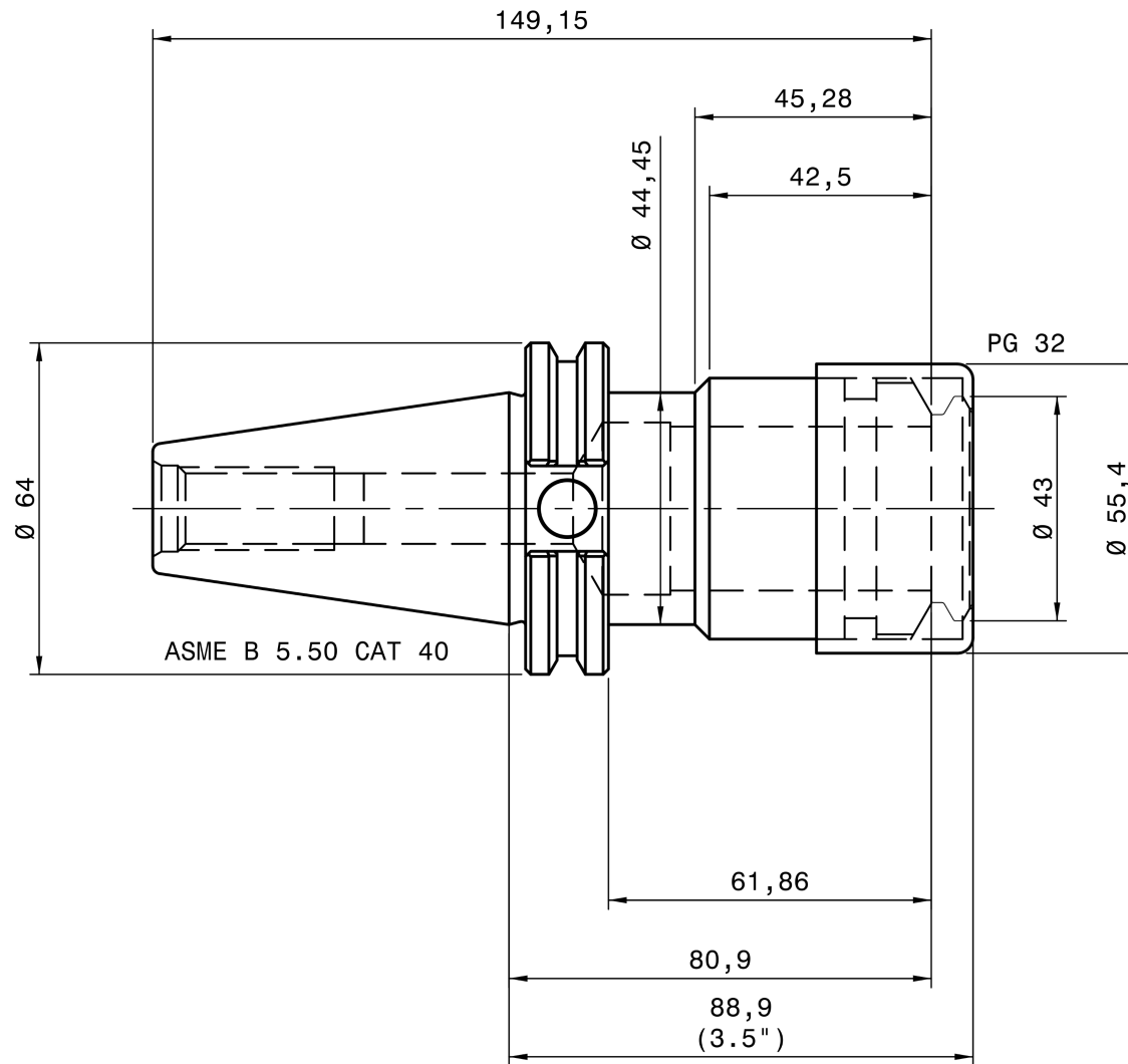
REGO-FIX SG 5340.73201
