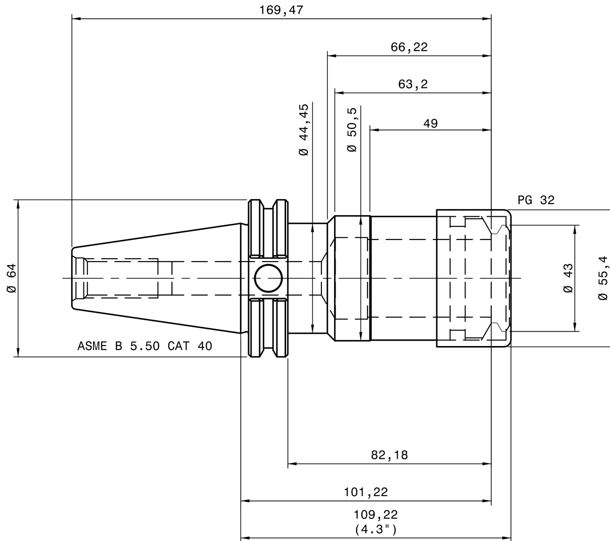
REGO-FIX SG 5340.73251
