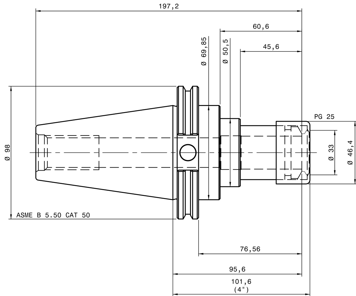
REGO-FIX SG 5350.72551
