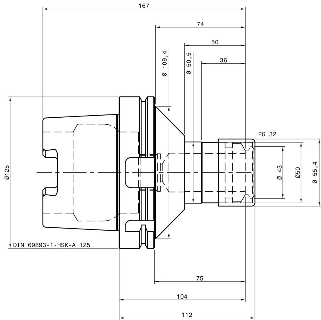
REGO-FIX SG 5502.83250
