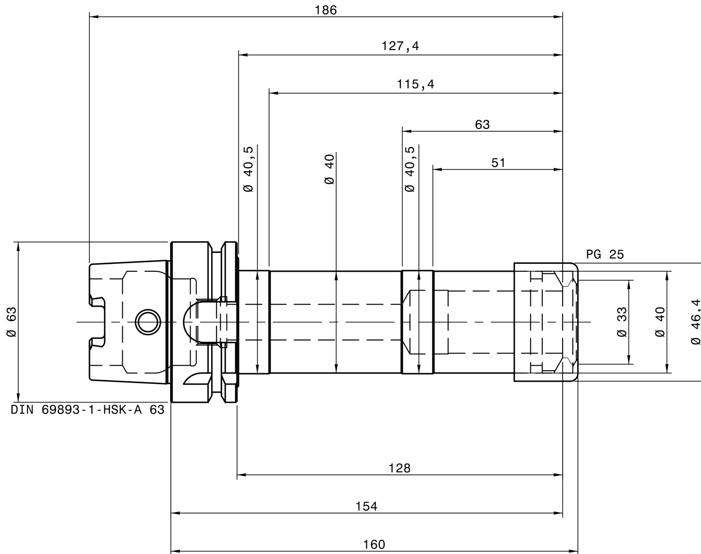
REGO-FIX SG 5563.72580
