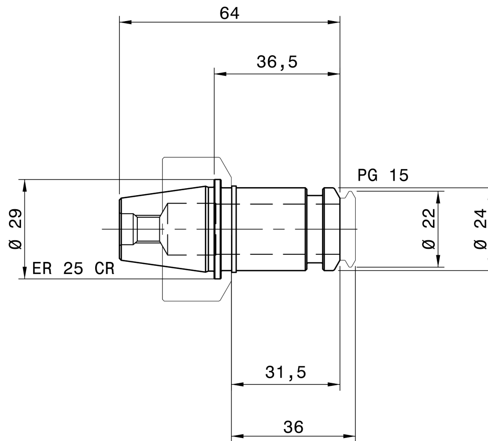
REGO-FIX 7660.25150
