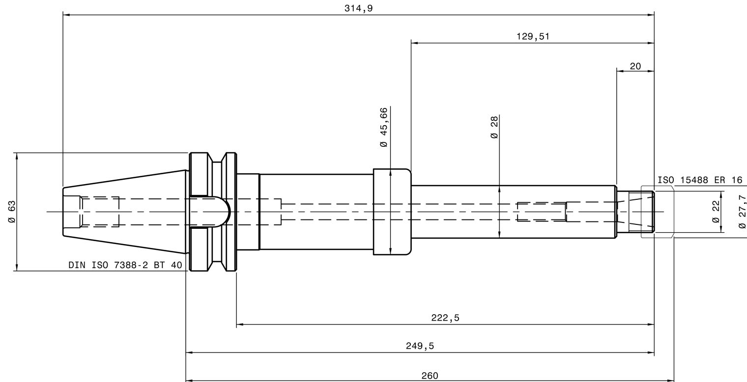
REGO-FIX 8841.13090
