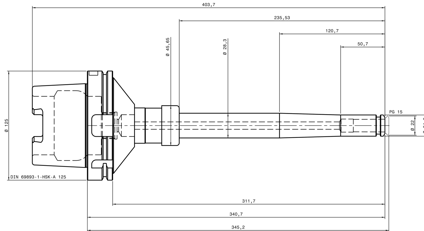
REGO-FIX 8895.73170
